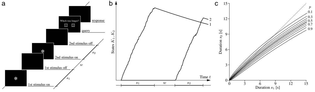
Figure 1. (a) Time chart of an experimental trial. (b) Sample trajectories of states accumulated at klepsydrae 1, 2. (c) Contour plot of a PMF with parameters \gamma = 3.162 \text{ s}^{-1/2} , \kappa = 0.02 \text{ s}^{-1} , w = 1 \text{ s} ; dotted line: physical equality \mathbf{I} \equiv \{s_1 = s_2\} ; thick curve: subjective equality \mathbf{E}_{1/2} .
