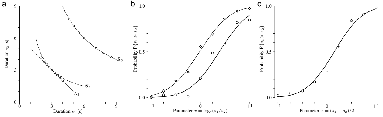
Figure 2. Experimental data on duration discrimination. (a) Stimuli employed in the two reported studies. (b) PMFs from the first study; thin curve, \diamond : short durations ( S_3 ), thick curve, \circ : long durations ( S_6 ); each data point based on 72 trials (9 subjects \times 8 repetitions). (c) PMF from the follow-up study; each data point based on 100 trials (10 subjects \times 10 repetitions).
