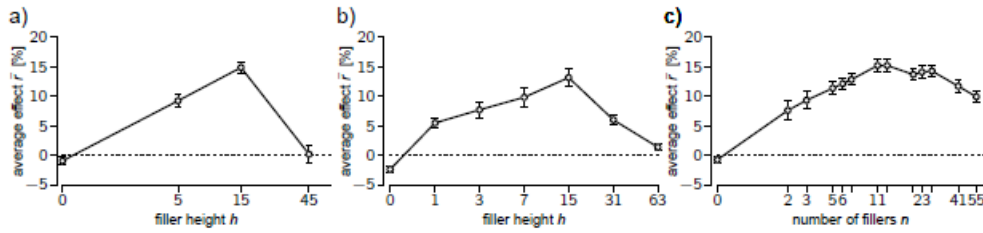
Figure 4. Results of studies 1–3. Average effects are plotted as functions of the respective control parameter, h or n (logarithmic scales). 0 = control task (empty space between S_0, S_1 ). Error bars indicate probable errors of the grand means.
